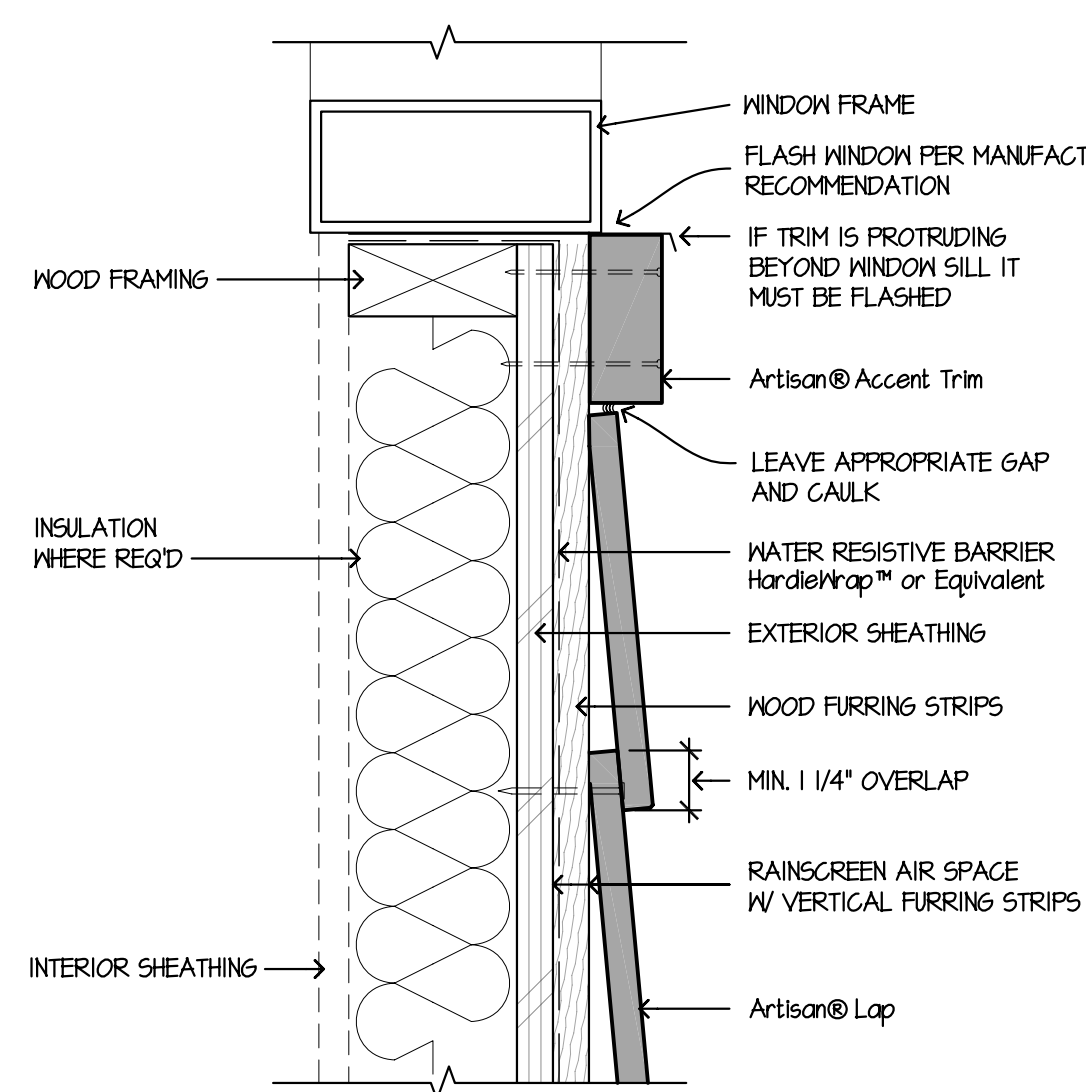
5 HORIZONTAL LAP VIEW - RAINSCREEN SCALE: 3/4"=1'-0"
