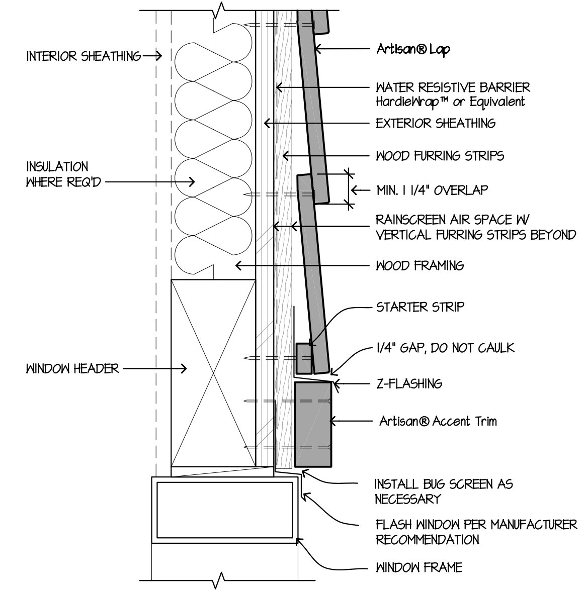
3 WINDOW/DOOR HEAD - RAINSCREEN SCALE: 3/4"=1'-0"
