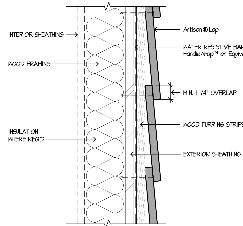
5 HORIZONTAL LAP VIEW - RAINSCREEN SCALE: 3/4"=1'-0"
