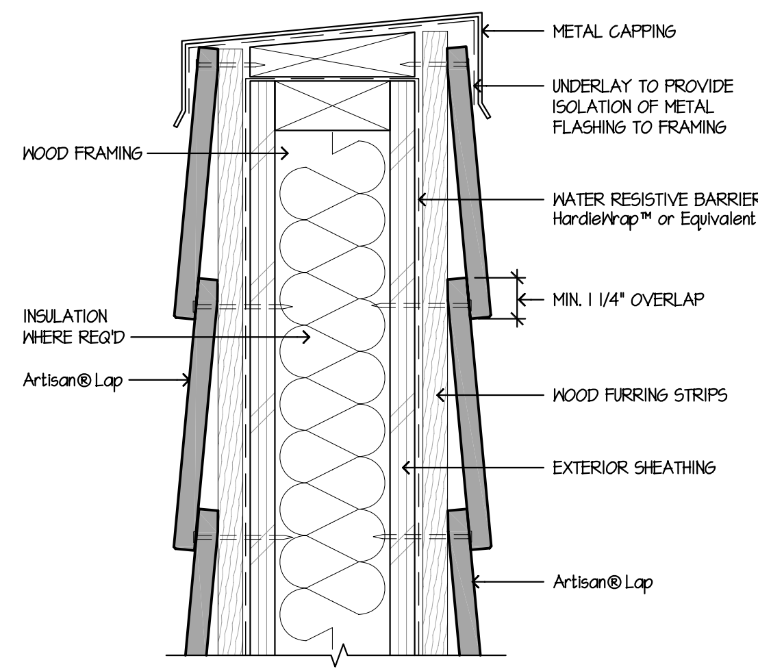
9 PARAPET - RAINSCREEN SCALE: 3/4"=1'-0"
