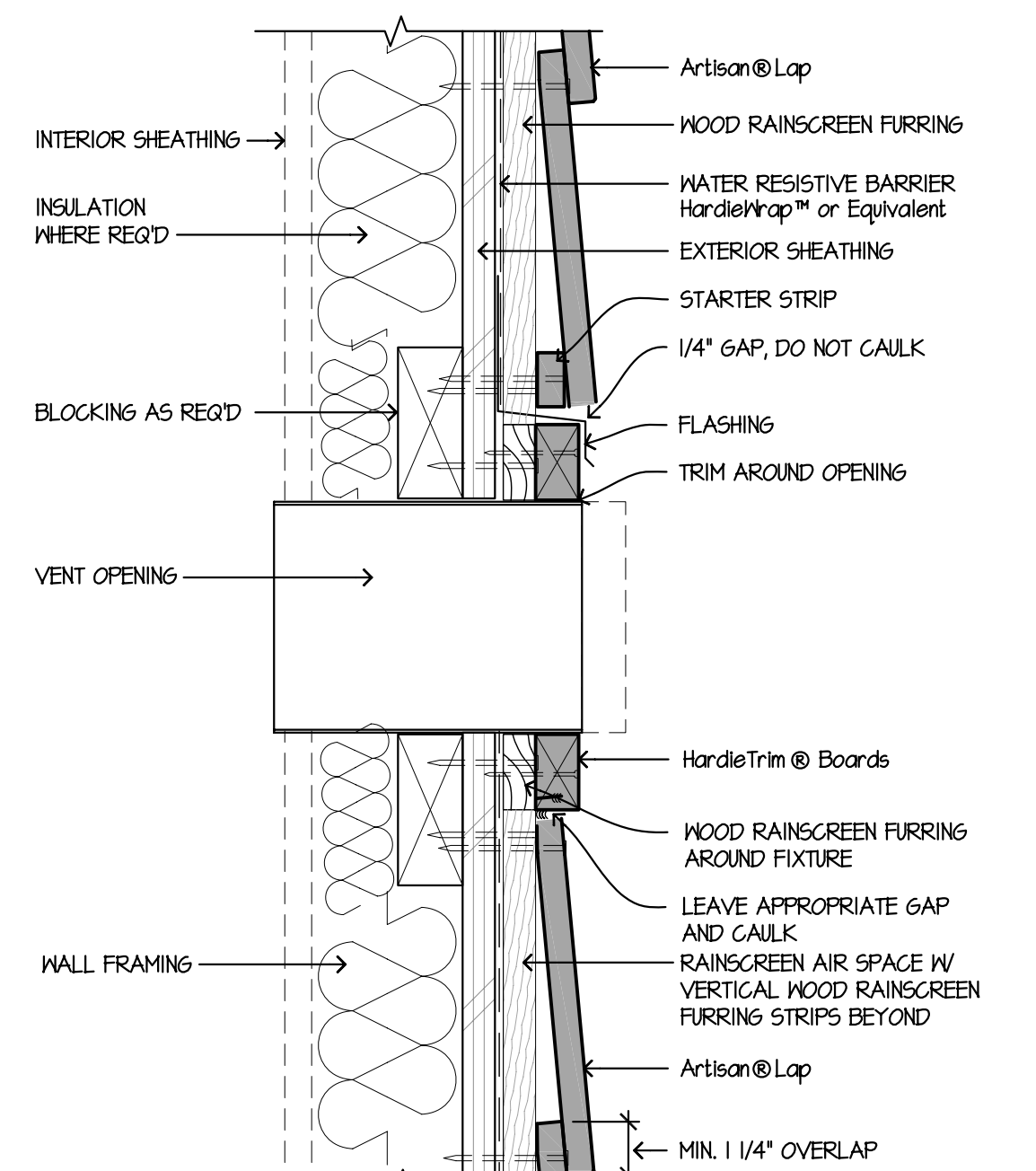
7 FIXTURE PENETRATION - RAINSCREEN SCALE: 3/4"=1'-0"
